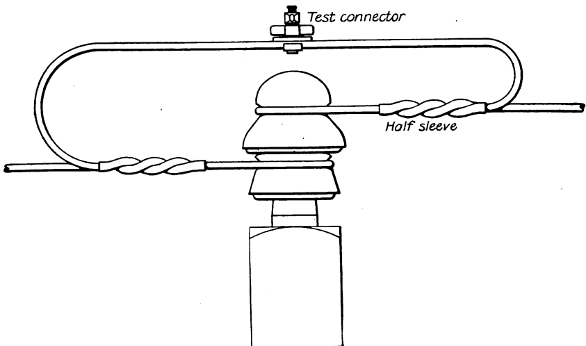
FIG. 127.—Test connector.
